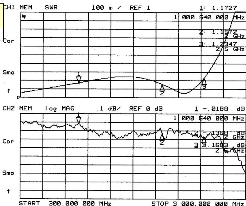
Typical RF Performance
